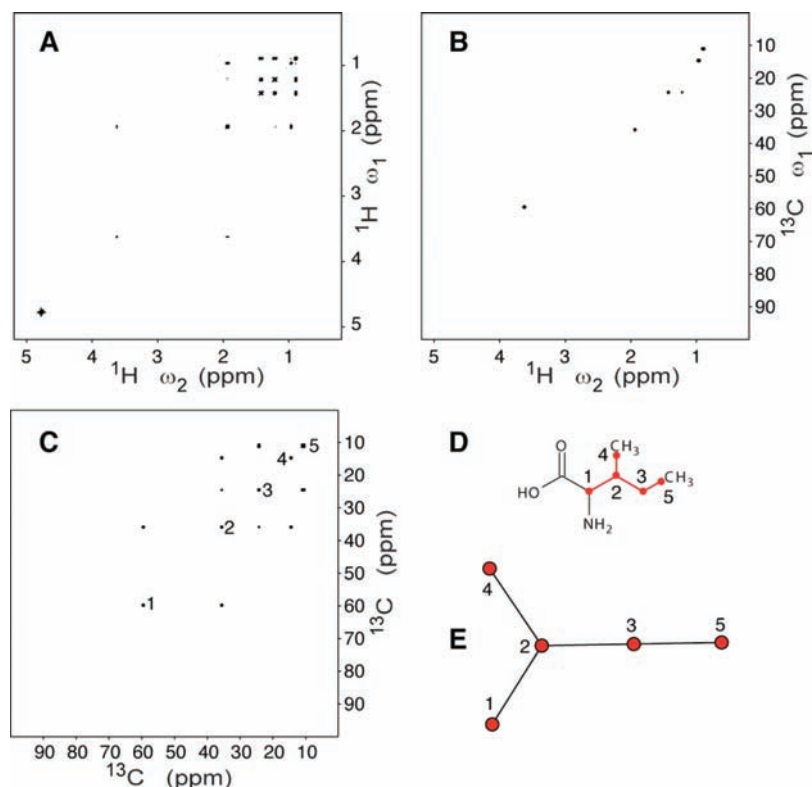
Figure 1. Carbon skeleton of isoleucine derived from doubly indirect covariance spectrum (C) constructed from (A) 2QF-COSY and (B) ^{13}\text{C}-^1\text{H} HSQC (see eq 2). (D) Chemical structure of isoleucine. (E) Graph theoretical representation of skeletal formula obtained from covariance spectrum. The carboxyl carbon is not included since it does not have a proton attached. Nodes 1, 2, and 3 represent \text{C}_\alpha , \text{C}_\beta , and \text{C}_{\gamma_1} , respectively, and nodes 4 and 5 represent the \text{CH}_3 groups of \text{C}_{\gamma_2} and \text{C}_{\delta_1} , respectively. All spectra were collected at 800 MHz proton frequency at 298 K. The chemical structures in this and the following figures were drawn using ChemSketch (Advanced Chemistry Development Inc., Toronto, Canada).
