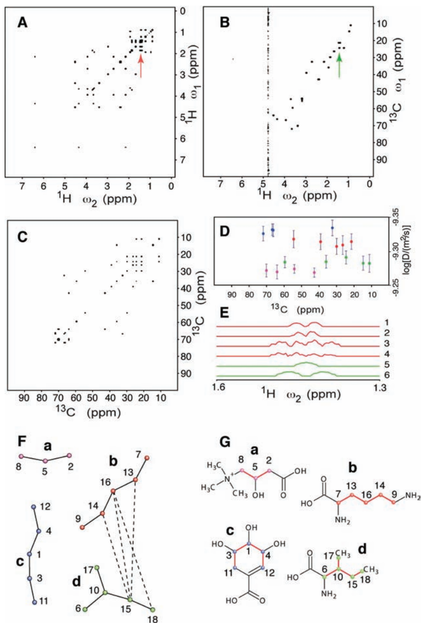
Figure 2. Doubly indirect covariance spectroscopy of model mixture containing carnitine, lysine, isoleucine, and shikimate. (A) 2QF-COSY spectrum, (B) ^{13}\text{C} - ^1\text{H} HSQC spectrum, (C) doubly indirect covariance spectrum (see eq 2), (D) INEPT DOSY spectrum, (E) absolute value cross sections along ^1\text{H} dimension of COSY and HSQC for the overlap \omega_2 = 1.45 ppm (traces 1–4 belong to COSY and traces 5,6 to HSQC). (F) Carbon–carbon connectivity graphs of mixture components. Dashed lines indicate extraneous connectivities to nodes 15 and 16 due to ^1\text{H} overlap at 1.45 ppm as indicated by arrows in panels A and B. They are identified based either on DOSY (panel D) or by filtering according to differential peak positions and shapes (panel E). The labels a, b, c, d in panels F and G belong to carnitine, lysine, shikimate, and isoleucine, respectively. The computational time on a workstation with a single-core processor is 19 s.
