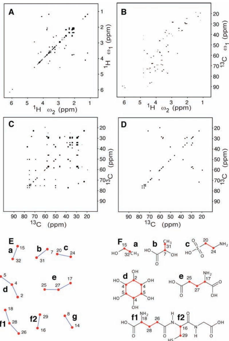
Figure 3. Doubly indirect covariance spectroscopy of cancer cell line DU145 extract. (A) 2QF-COSY spectrum, (B) ^{13}\text{C} - ^1\text{H} HSQC spectrum, (C,D) doubly indirect ^{13}\text{C} - ^{13}\text{C} covariance spectrum constructed from parent spectra A, B (see eq 2) before (C) and after (D) removing effects due to ^1\text{H} overlap, (E) carbon-carbon connectivity graphs of mixture components determined from spectrum D. (F) Labels a, b, c, d, e, f1, and f2 in panels E, F indicate ethanol, lactate, taurine, myo-inositol, glutamate, and glutathione reduced, respectively. Graph g in panel E does not match any of the compounds in the database. Myo-inositol displays only three nodes (graph d in panel E) because of ^{13}\text{C} chemical shift degeneracy induced by its molecular symmetry.
